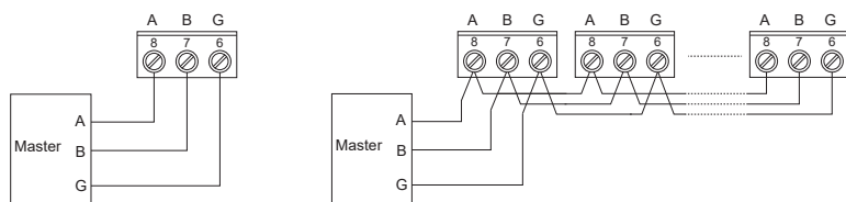
Single meter wiring
