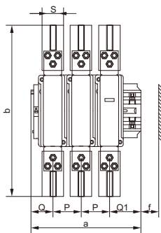
T type overall dimension
