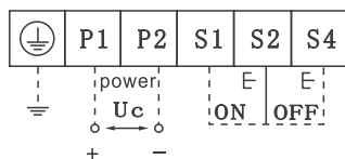
AC wiring diagram 2
