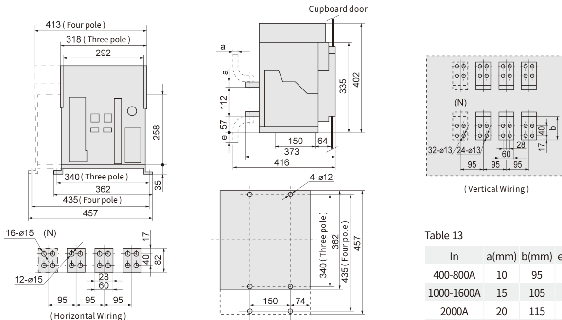
Fig.10 Outline and installation dimensions of fixed type circuit breaker (EKA1-2000, 2000/4)
